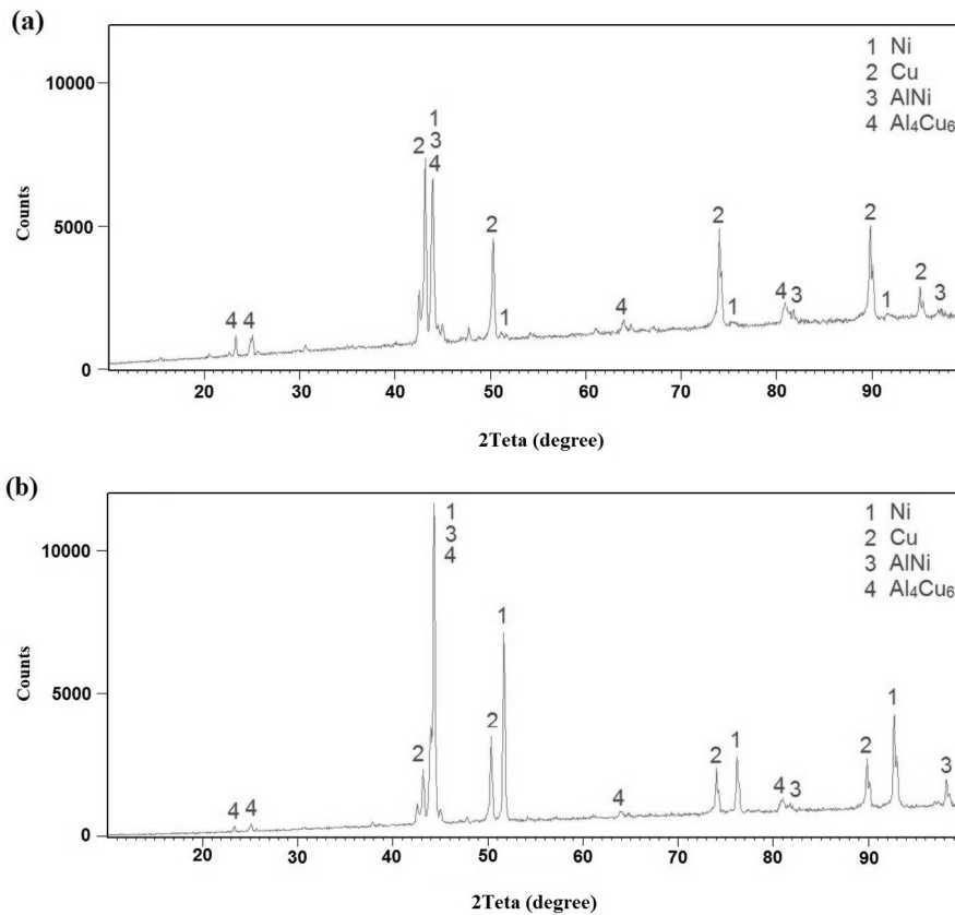
Fig. 5. Typical X-ray diffraction patterns of 1 \times 1 \text{ cm}^2 of the Cu fractured surface for 50% reduction and 2 hours annealing at 773 K in the presence of (a) nickel powder and (b) nickel coating.
