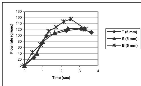
Fig. 17. Effect of the gating system on mold filling in 5 mm thickness
