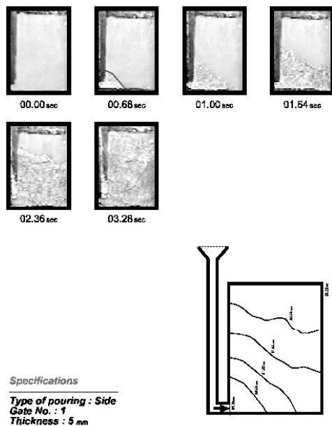
Fig. 5. Mold filling sequences in the side pouring of a 5 mm thick plate in the LFC process
