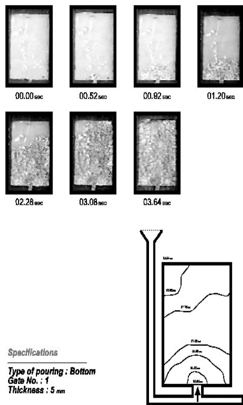
Fig. 7. Mold filling sequences in the bottom pouring of a 5 mm thick plate in the LFC process
