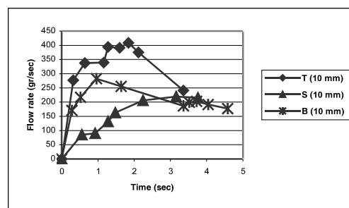
Fig. 18. Effect of the gating system on mold filling in 10 mm thickness
