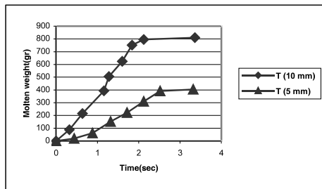
Fig. 9. Effect of the pattern geometry on mold filling in top gating system
