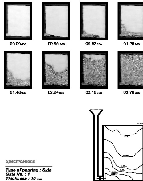
Mold filling behavior of 413 Aluminium Alloy in lost foam casting.
