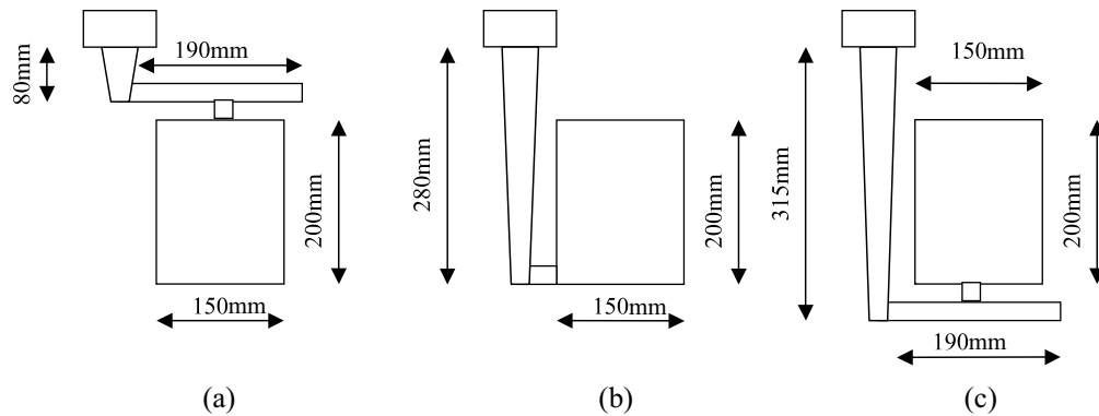
Fig. 1. Schematic illustration of the gating systems: (a) top gating. (b) side gating (c) bottom gating
