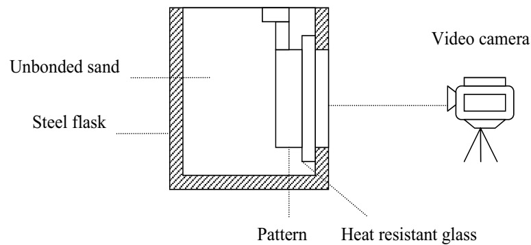
Fig. 2. Schematic of the experiment method
