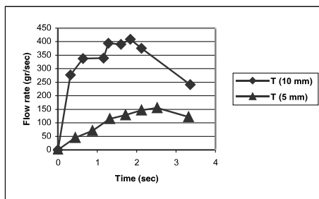
Fig. 11. Effect of the pattern geometry on mold filling in top gating system
