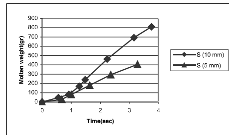
Fig. 10. Effect of the pattern geometry on mold filling in side gating system
