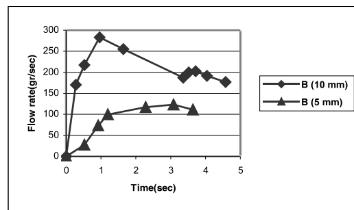
Fig. 14. Effect of the pattern geometry on mold filling in bottom gating system
