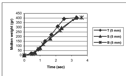
Fig. 15. Effect of the gating system on mold filling in 5mm thickness
