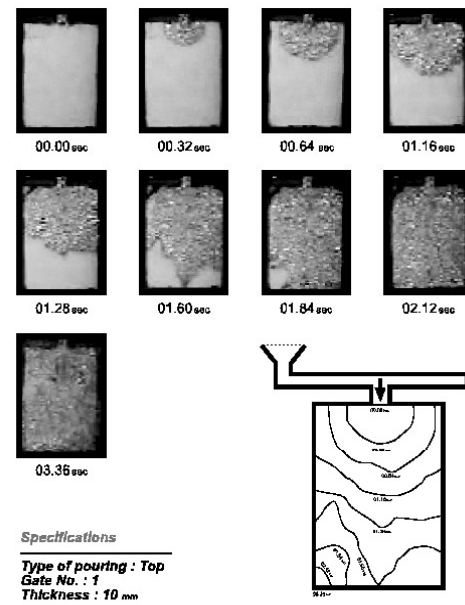
Fig. 4. Mold filling sequences in the top pouring of a 10 mm thick plate in the LFC process
