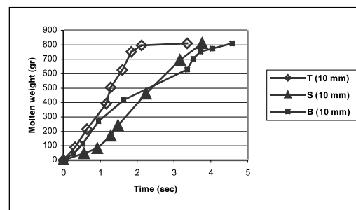
Fig. 16. Effect of the gating system on mold filling in 10 mm thickness
