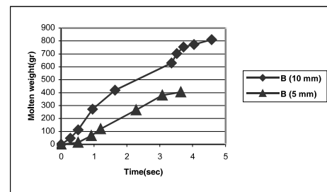
Fig. 10. Effect of the pattern geometry on mold filling in side gating system
