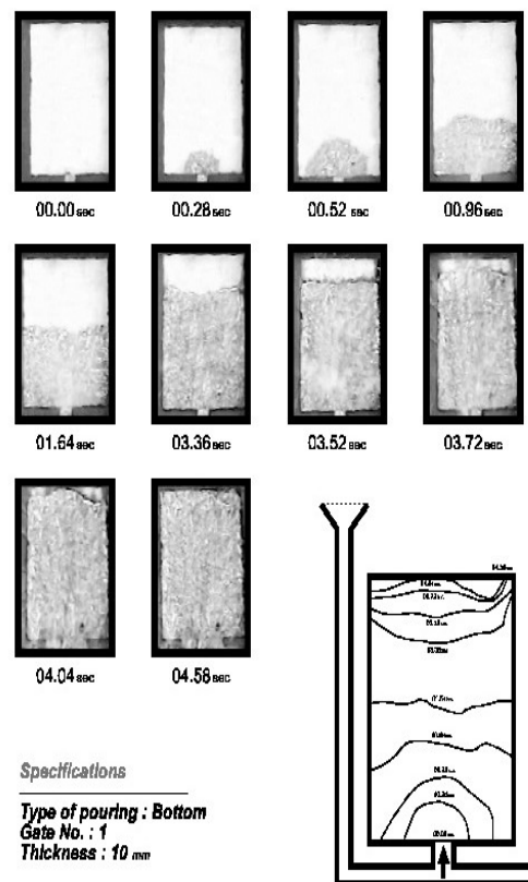
Fig. 8. Mold filling sequences in the bottom pouring of a 10 mm thick plate in the LFC process
