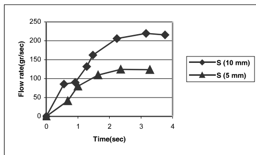
Fig. 13. Effect of the pattern geometry on mold filling in side gating system
