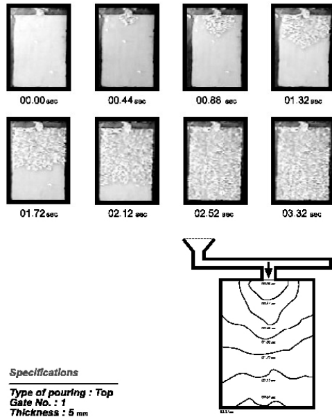
Fig. 3. Mold filling sequences in the top pouring of a 5 mm thick plate in the LFC process
