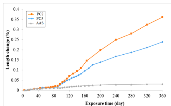
Fig. 7. Length change of PC2, PC5, and AAS mortar bars versus exposure time to sodium sulfate solution.
