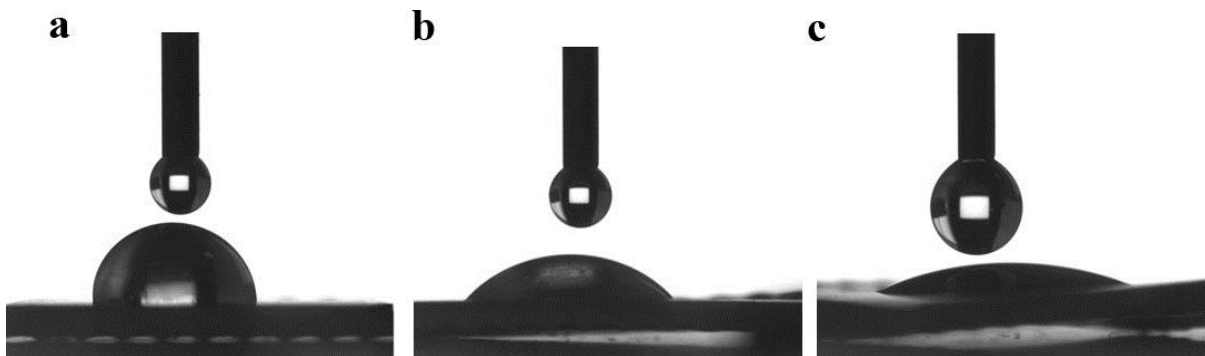
Fig. 6. Fig. 6-Contact angle of a human blood droplet on the surface of a titanium sheet a) 85° average for Coated with titanium oxide b) 44° average on Coated with titanium oxide nanotube c) 26° average angle on Coated with heat-treated titanium oxide nanotube.
