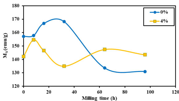
Fig. 12. Variations of saturation magnetization versus milling time for Fe_{80}Ni_{20} and (Fe_{80}Ni_{20})_{96}Cr_4
