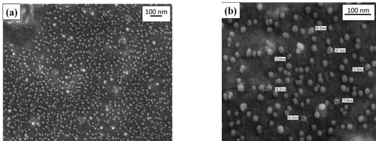
Fig. 4. FESEM image of EBN-AgNPs in 80\times (a) and 200\times (b).
