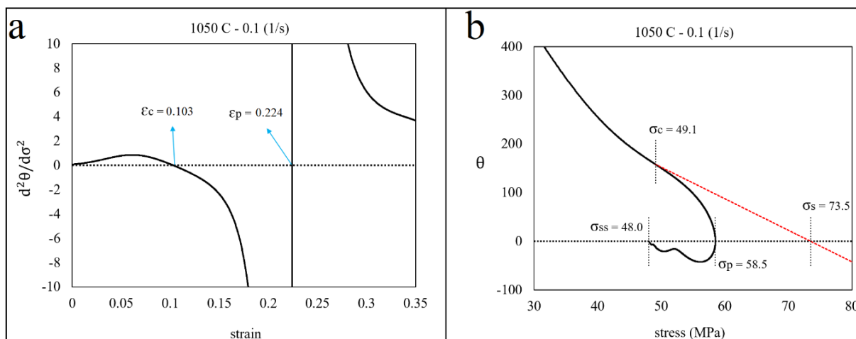
Fig. 6. a) d^2\theta/d\sigma^2 curve in terms of strain, b) \theta - \sigma curve, for the hot compression test sample at 1050°C and a strain rate of 0.1 s -1
