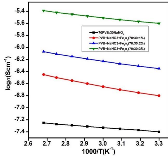
Fig. 6. Plots of log \sigma vs 1000/T for 70PVB+30 NaNO 3 and PVB+NaNO 3 +Fe 2 O 3 at various weight percent ratios.
