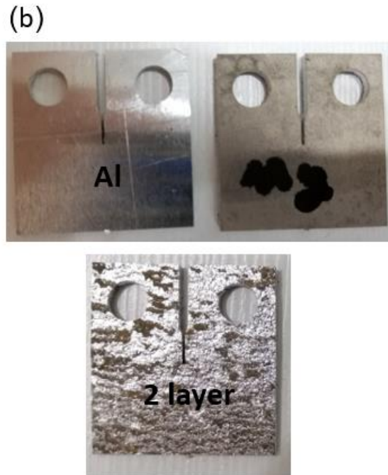
Fig. 3. a) Sample size, b) fracture toughness sample
