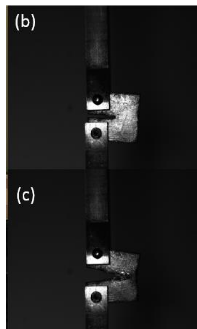
Fig. 4. a).Setup of the fracture toughness, b) before start test, C) end test
