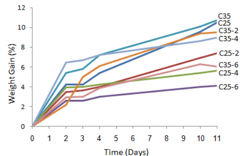
Fig. 8. Relationship between weight gain (%) from hydration and hydration duration (days) (conditions: 70% humidity and 110 °C)
