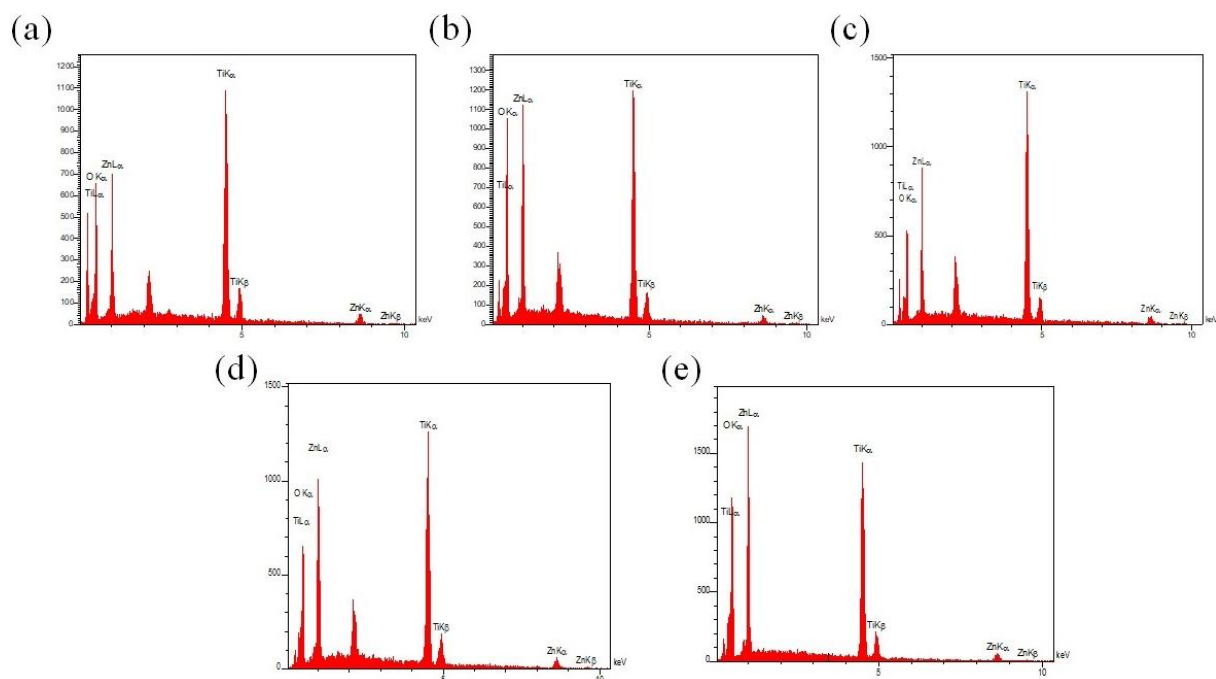
Fig. 4. The EDXS pattern of the TiO 2 -ZnO nanocomposites prepared at the times of (a) 1, (b) 1.5, (c) 2, (d) 2.5, and (e) 3 hour (s)
