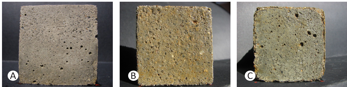
Fig. 3. PC5 mortar specimens exposed to sodium sulfate solution after A: 70 days, B: 140 days, and C: 280 days.
