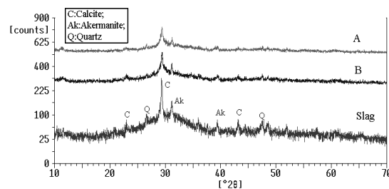
Fig. 4. X-Ray diffraction patterns of Slag, specimen cured at 95% R.H. at 25°C (specimen A), and specimen cured hydrothermally (specimen B) showing maximum compressive strength.
