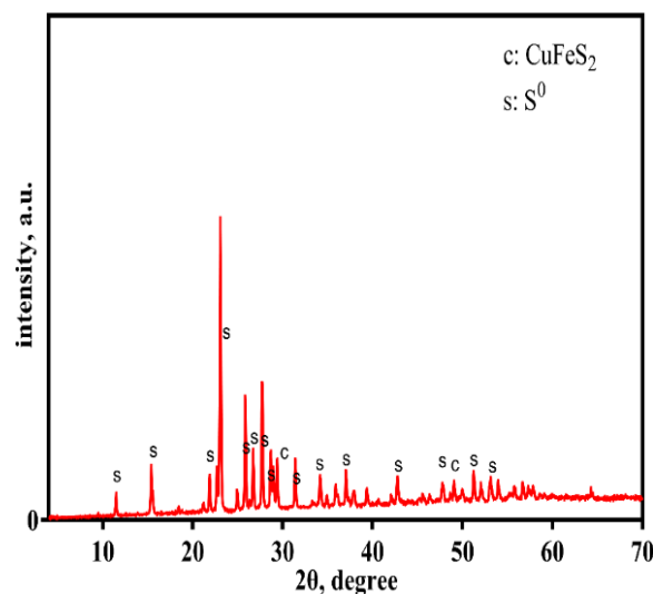
Fig. 10. XRD pattern of leached sample (40% \text{BmimHSO}_4 , 30% \text{H}_2\text{O}_2 , 10 g.L -1 solid to liquid ratio, stirring speed of 300 rpm, 45°C, particle size of under 37 \mu\text{m} , and leaching time of 180 min).
