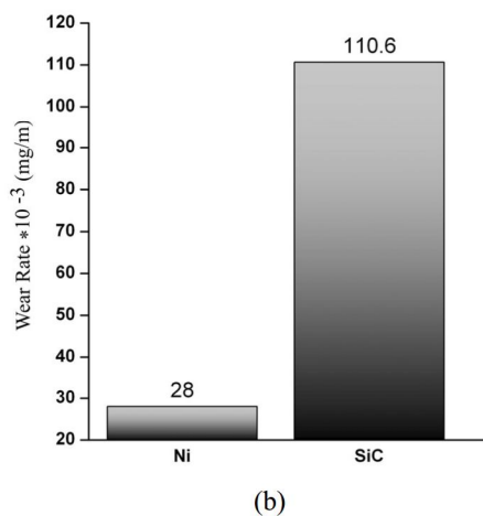
Fig. 6. (a) Friction coefficient and (b) wear rate of Ni and SiC coatings.
