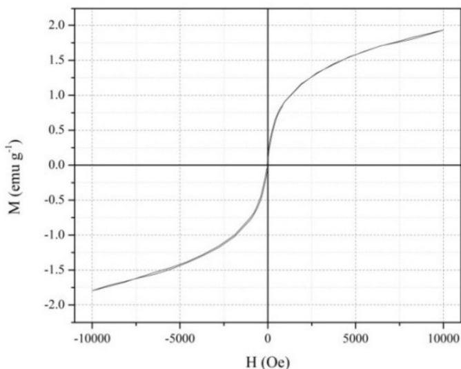
Fig. 3. Hysteresis loop of sample glass.
