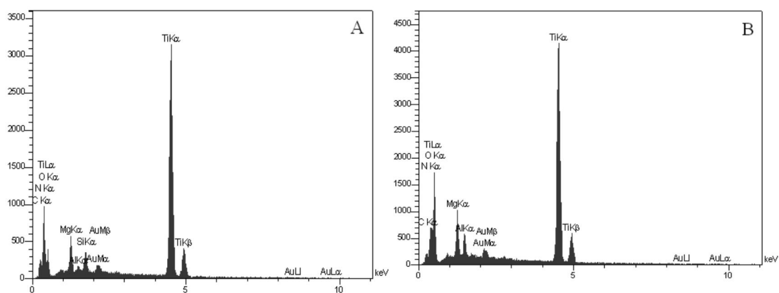
Fig. 6. Micrograph of EC sample after fired at 1600°C A) EDX of A point B)EDX of B point
