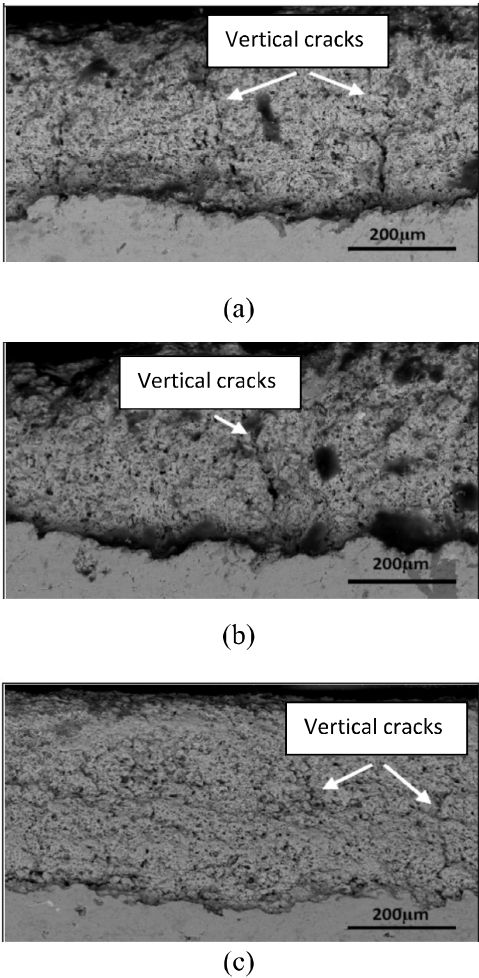
Fig. 8. SEM images from the section of coatings produced under the condition of test 2 at spray distances of 6 cm (a) and 16 cm (b) and test 3 at spray distance of 6 cm.
